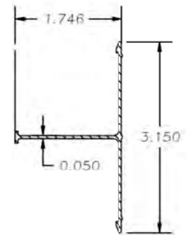
"T" ALUMINUM INSERT
